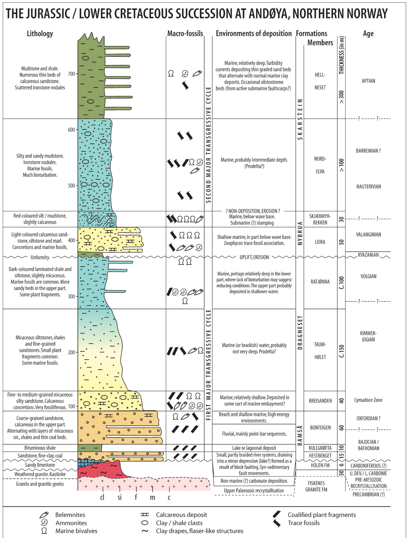
Figure 3. The Mesozoic sedimentary succession on Andøya. Only the lower part of the Lower Cretaceous Hellneset Member is shown. Redrawn from Dalland (1981).
